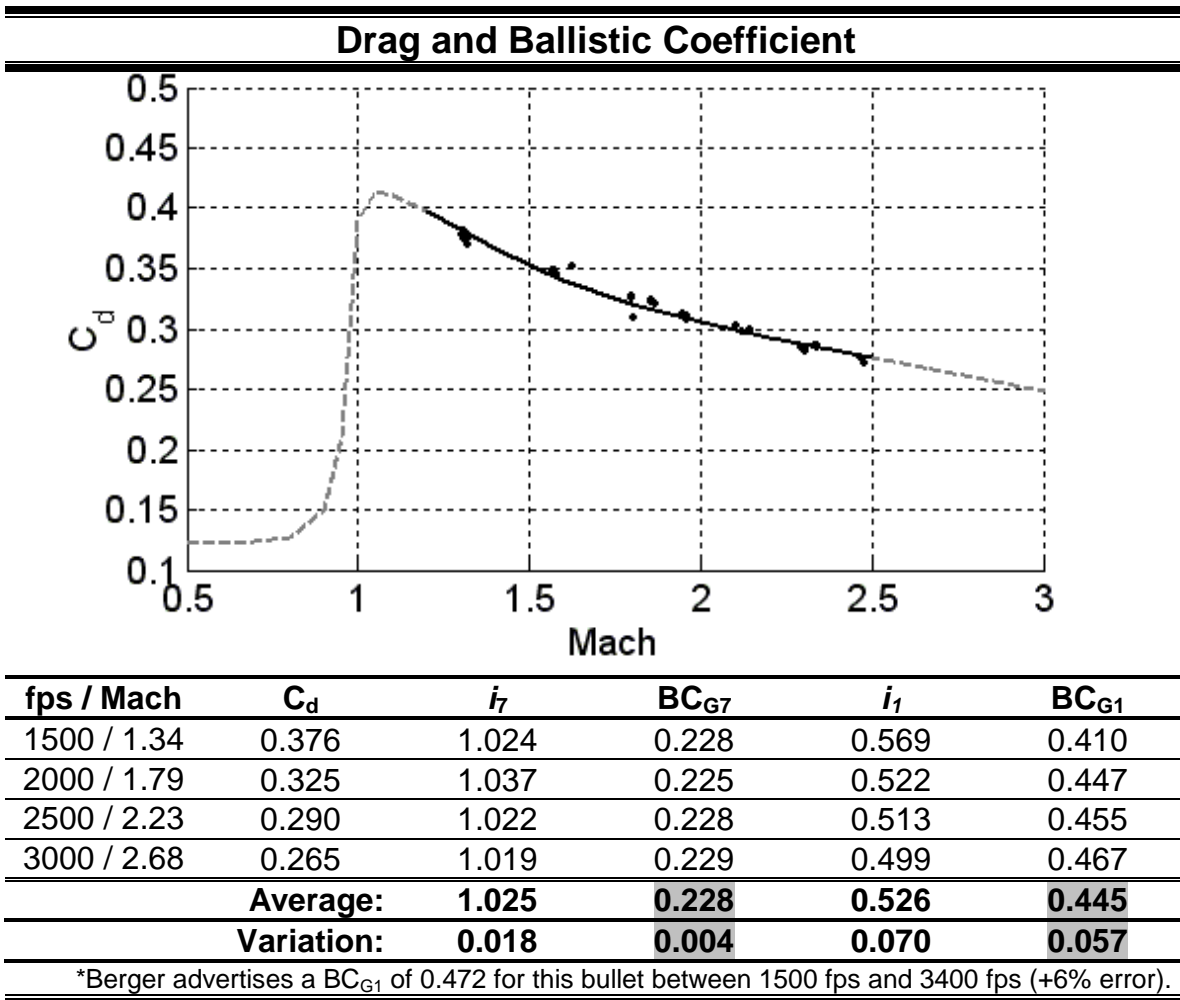
Figure 4. Drag and ballistic coefficient
